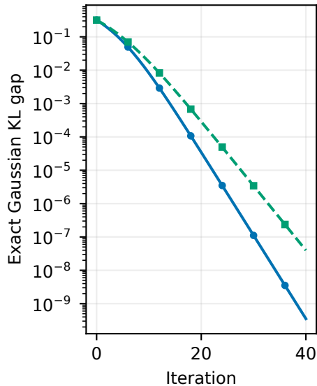
(b) Exact Gaussian local trajectory (c) Spectral-rate pilot
