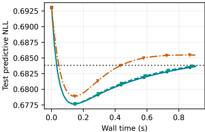
(c) Predictive loss versus wall time
