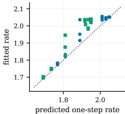
(c) Near-Gaussian \gamma_*
