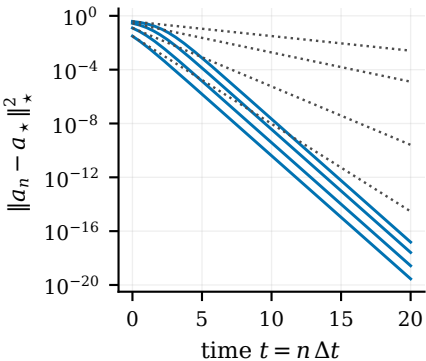
(a) Exact Gaussian region
