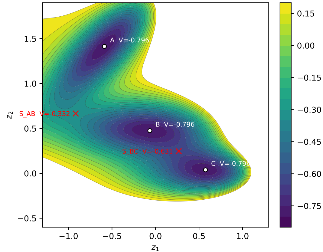
latent potential V_3(z_1, z_2) (depth-retuned)
