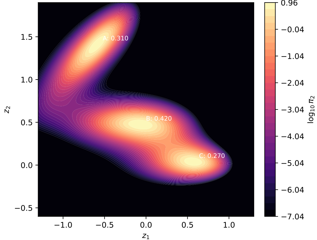
2D marginal \log_{10} \pi_2 at \beta = 24 (labels: basin masses)
