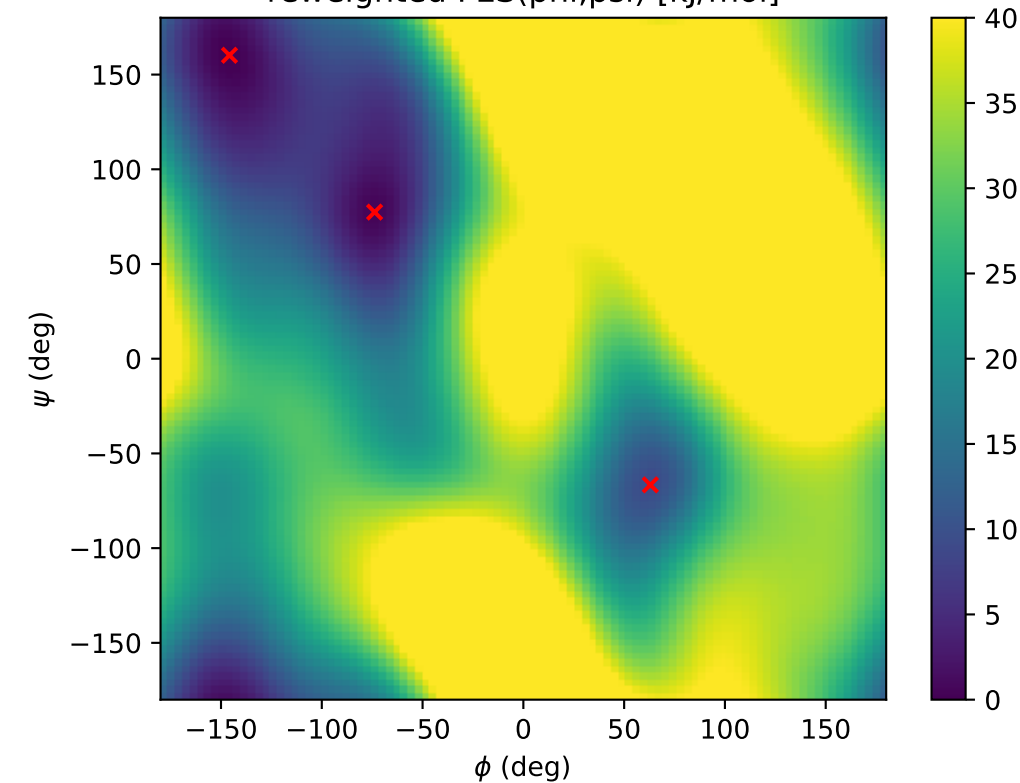
reweighted FES( \phi , \psi ) [kJ/mol]
