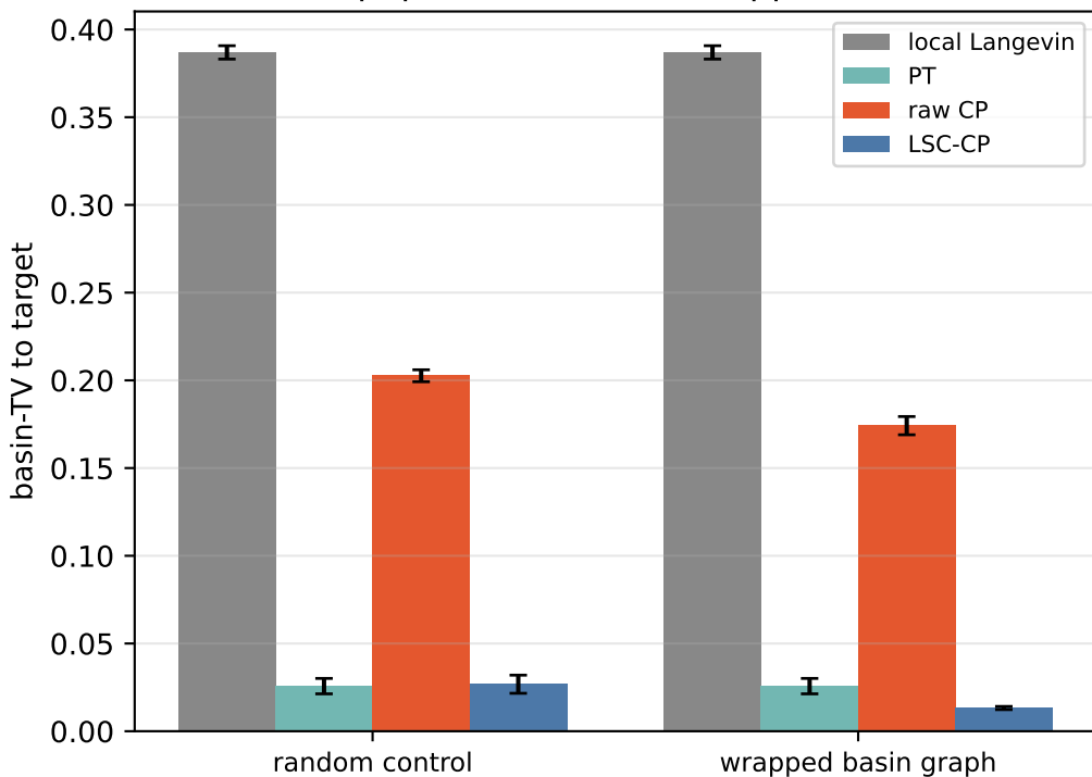
Alanine dipeptide: basin-TV (wrapped vs random)
