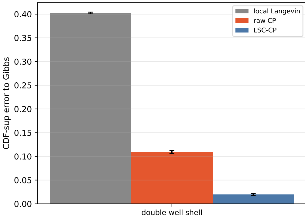
Double well: target fidelity
