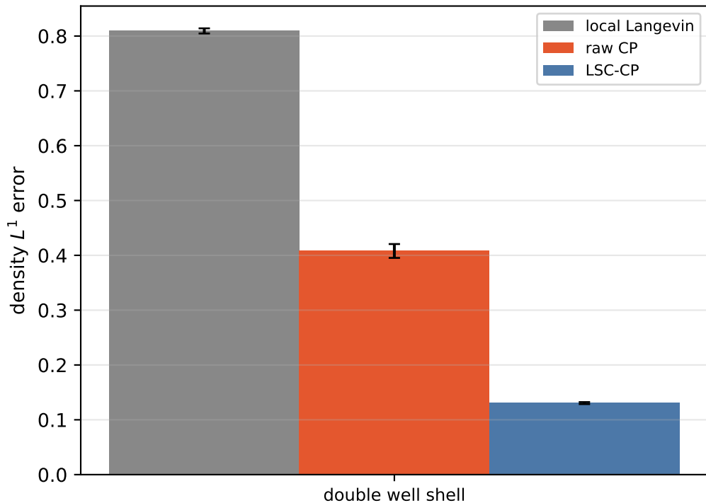
Double well: density error
