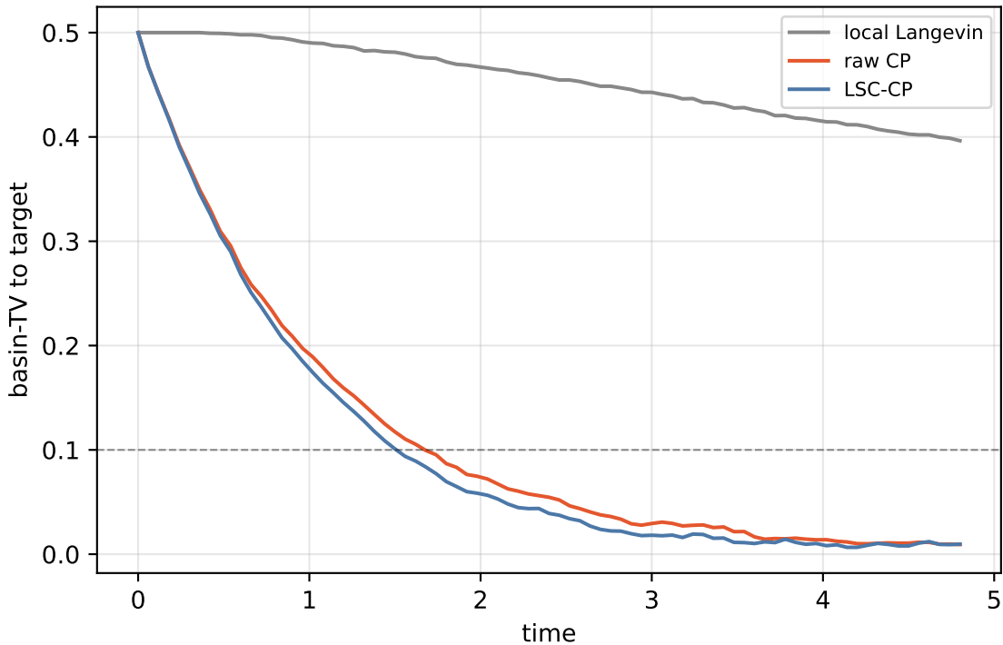
Double well: TV relaxation
