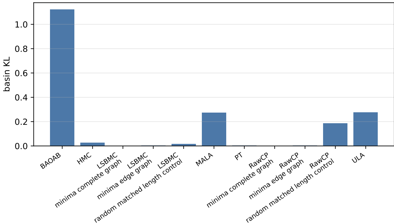
Four well: basin KL
