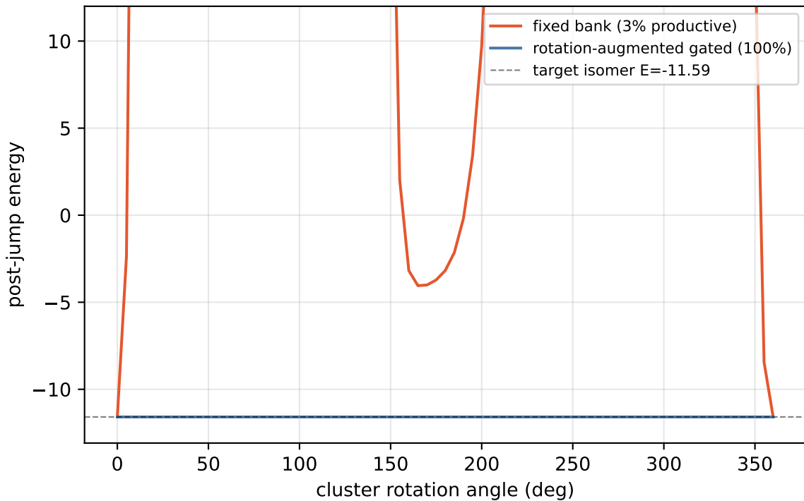
LJ 7 obstruction: fixed jumps break under rotation
