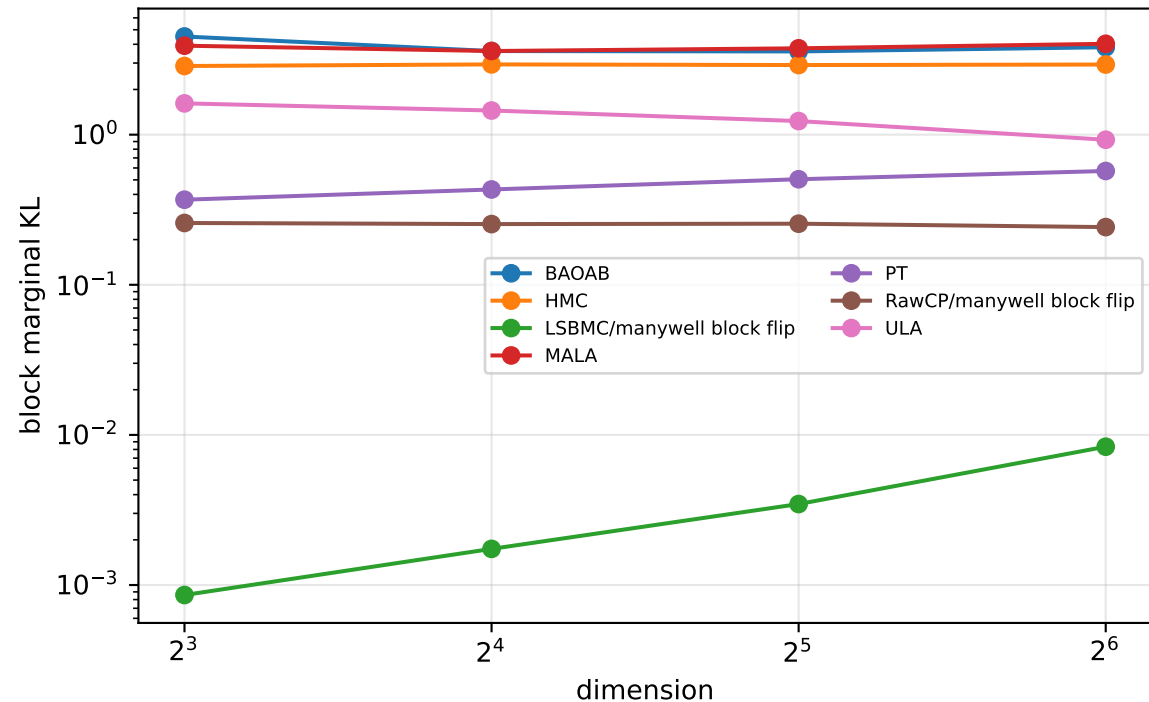
ManyWell scaling: block marginal KL
