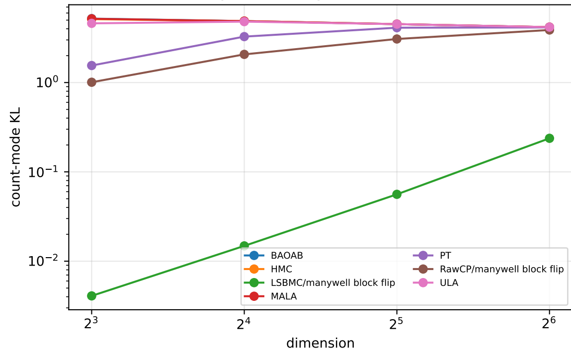
ManyWell scaling: count-mode KL
