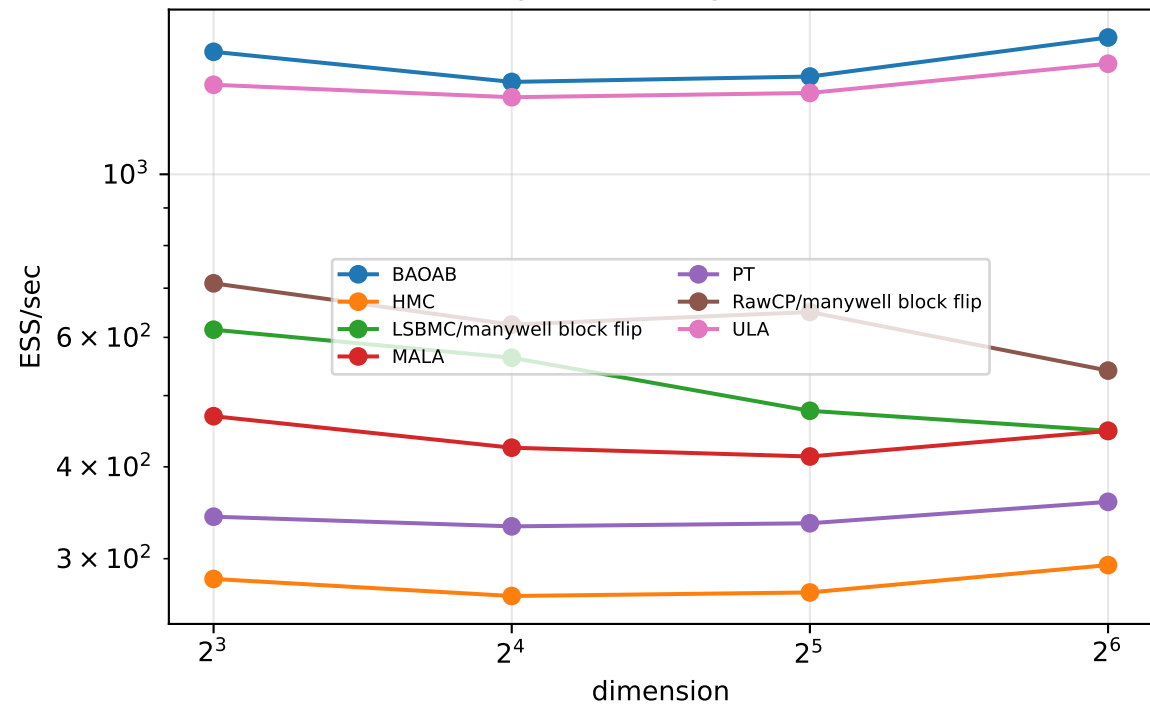
ManyWell scaling: ESS/sec
