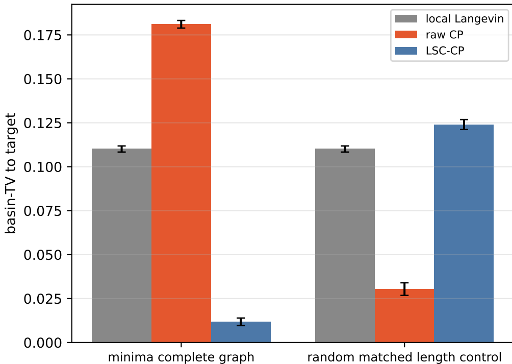
10D Muller-Brown: basin-TV (lifted vs random)
