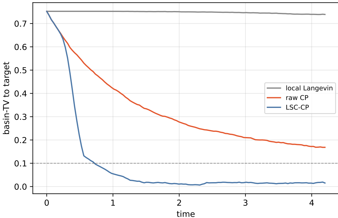
Triple well: TV relaxation (overlong)
