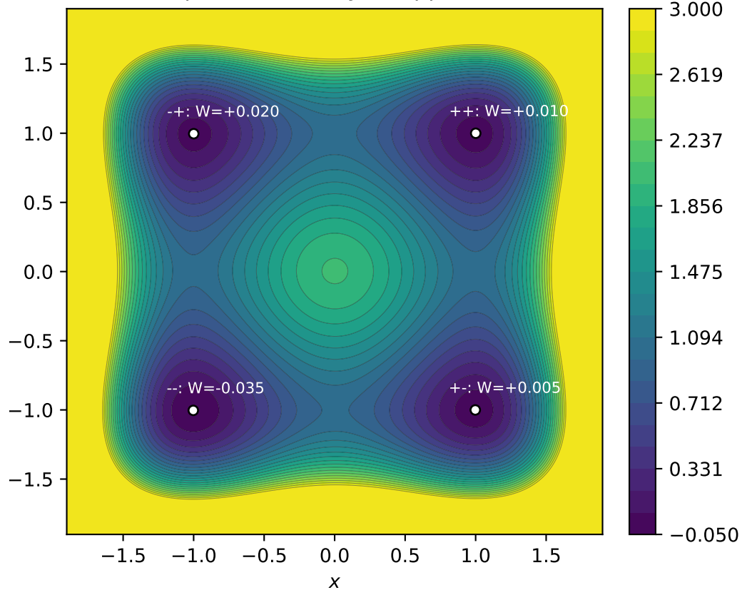
site potential W(x, y) (clipped at 3)
