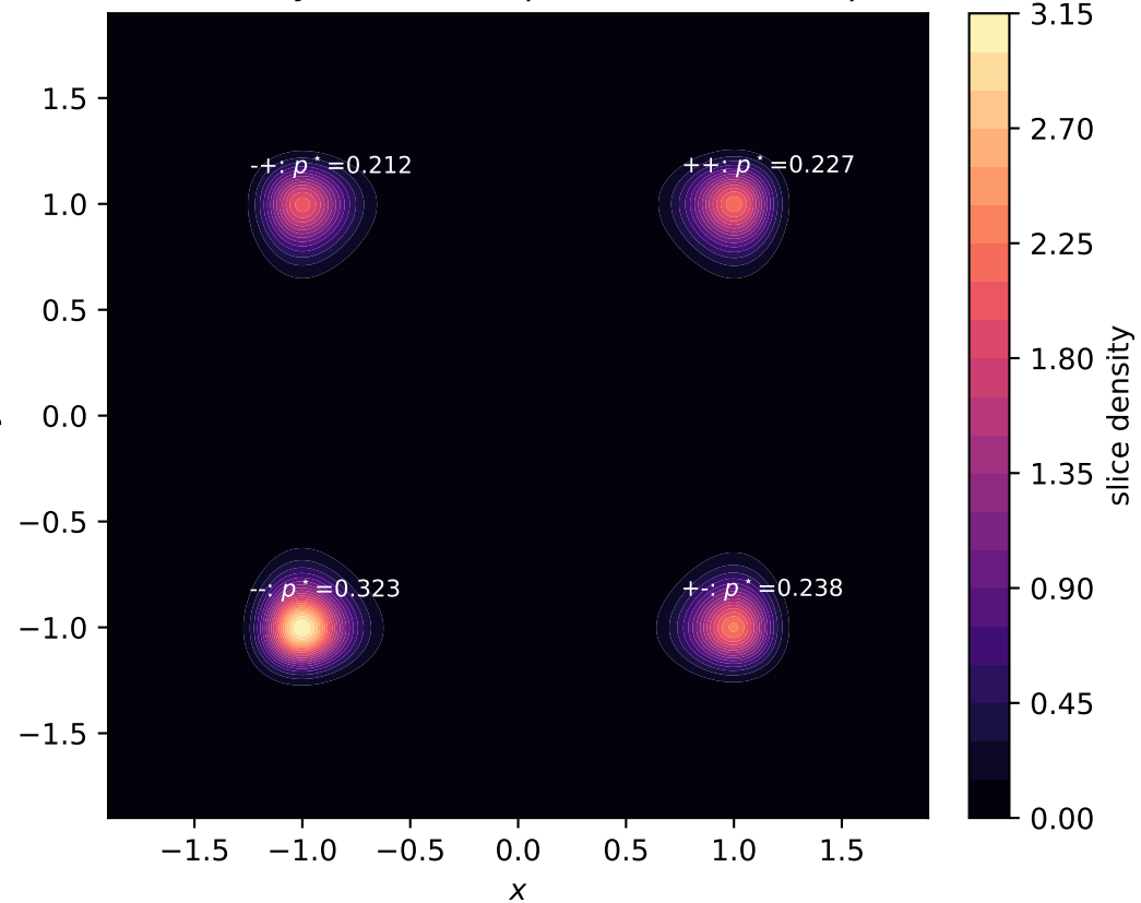
coherent-slice density e^{-\beta W}/Z_W at \beta = 8 (labels: 24D phase masses)
