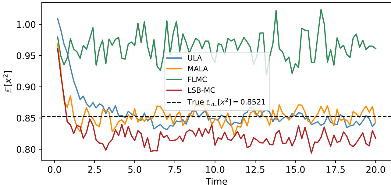
Test function \mathbb{E}[x^2] over time ( \sigma = 0.5 , dt = 0.01 , N = 2000 particles)
