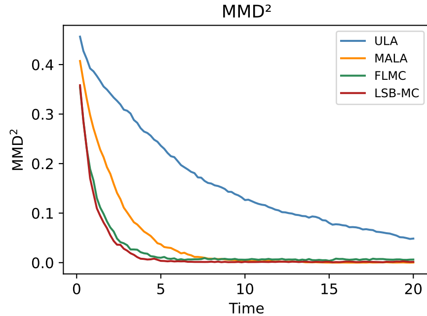
Double-well benchmark ( \sigma = 0.5 , dt = 0.01 , N = 2000 )
