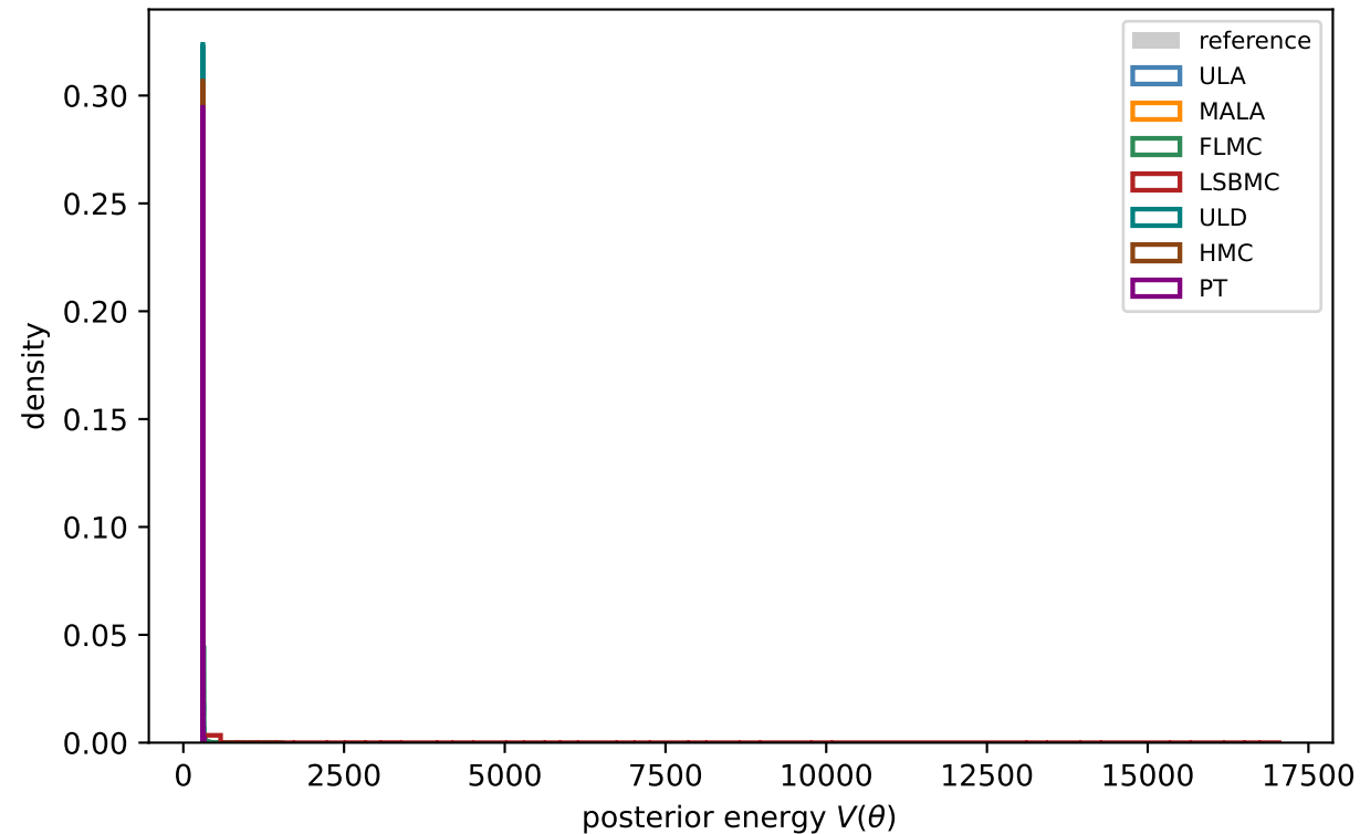
Bayesian GMM: posterior energy distribution
