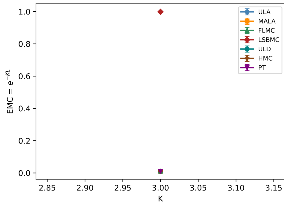
EMC = e^{-KL}
