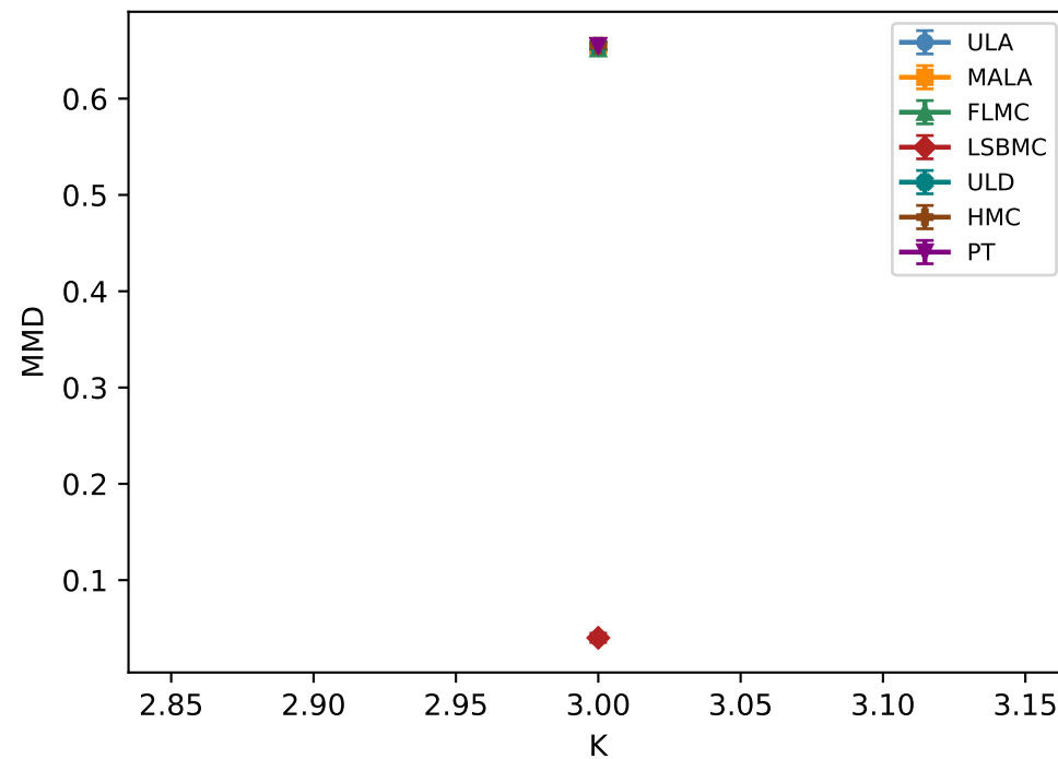
MMD
