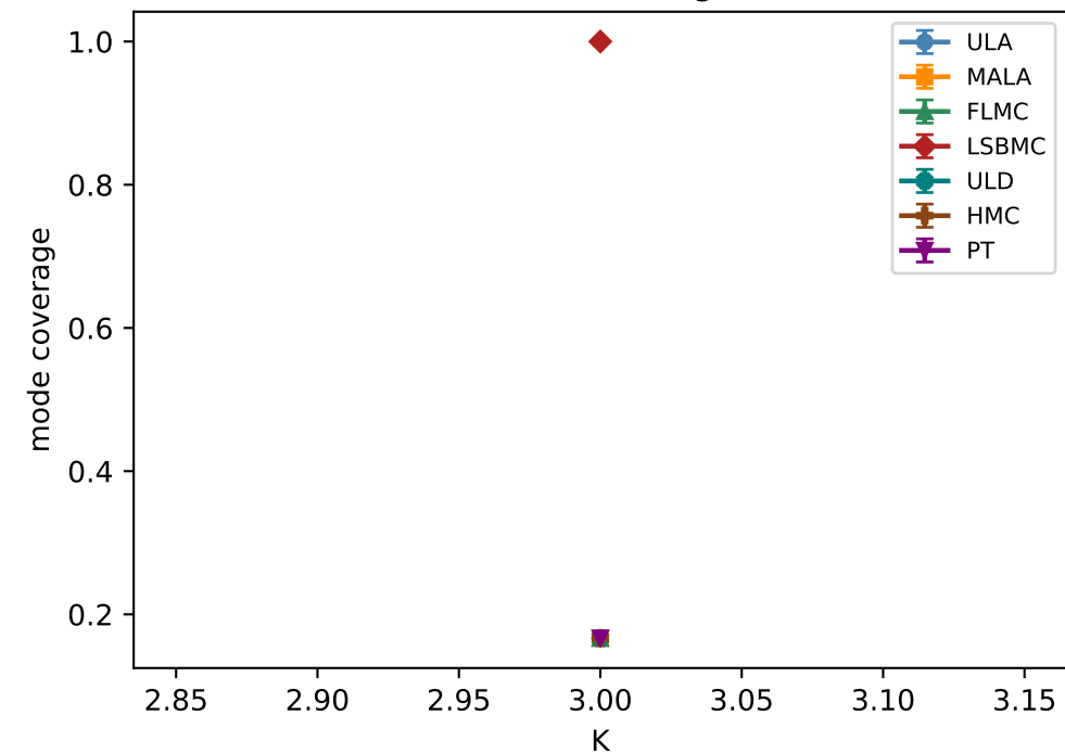
mode coverage
