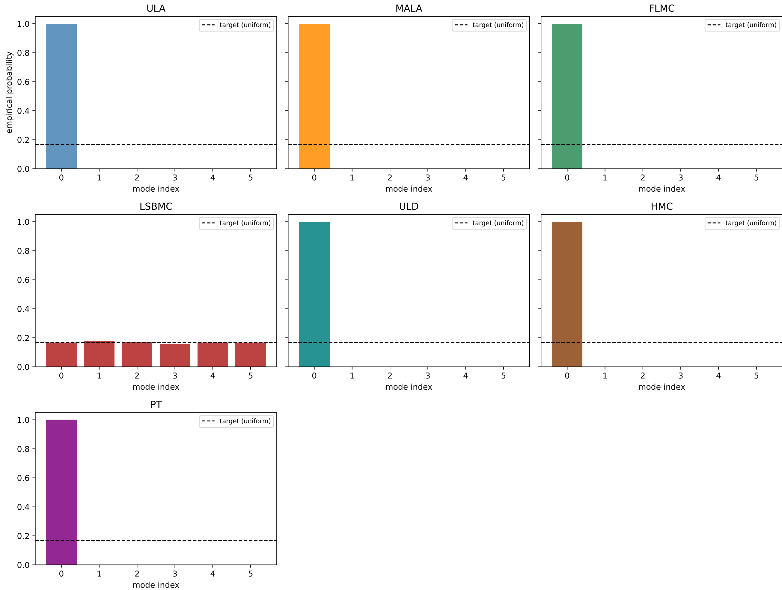
Bayesian GMM: empirical weight on each of the 6 label-permutation modes vs uniform
