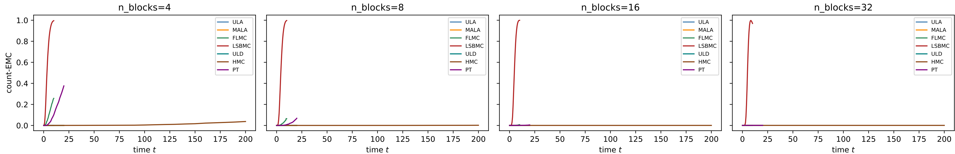
ManyWell: count-EMC over time
