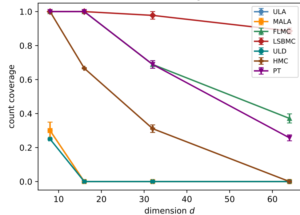
count coverage
