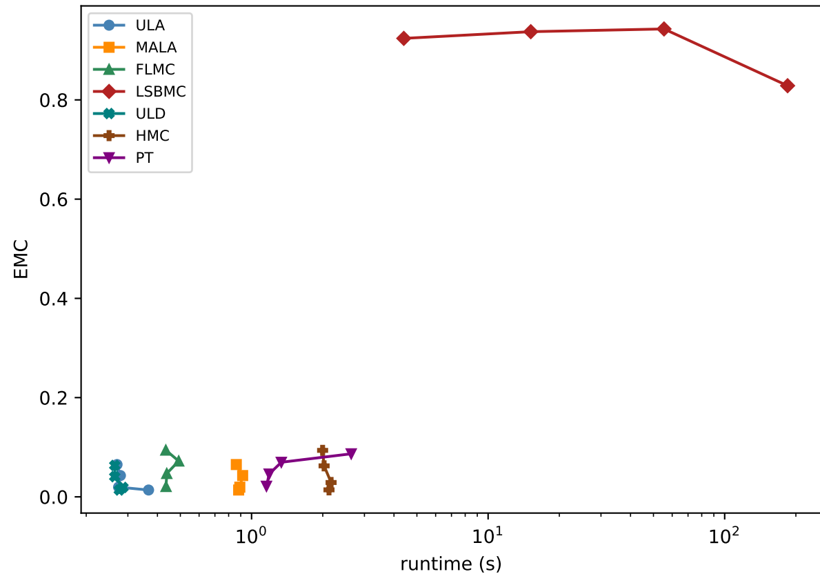
MoG: EMC vs wall-clock
