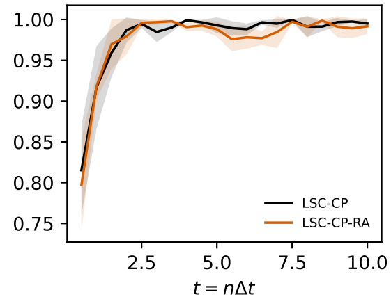
EMC
