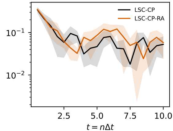
MMD
