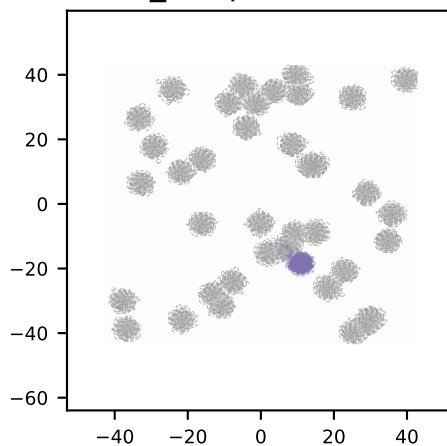
PT n_swap=10, tamed
