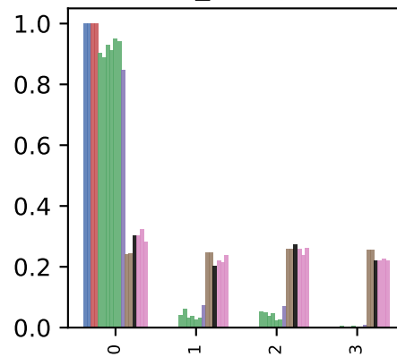
phase_occupancy
