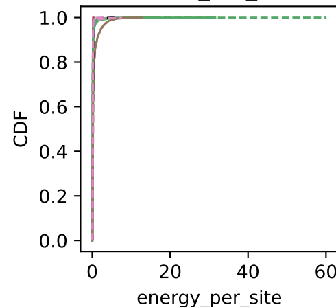
two_point_correlation
