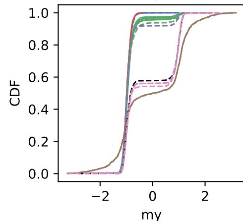
energy_per_site
