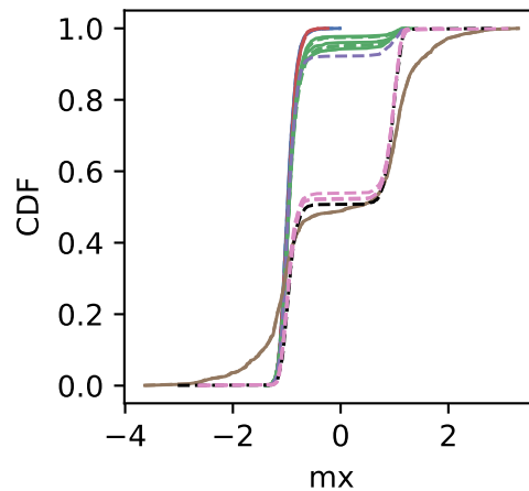
phase_occupancy
