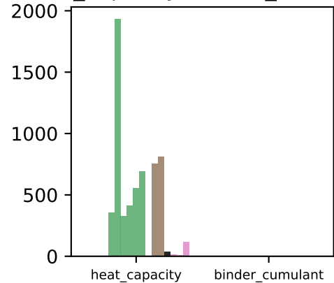
heat_capacity, binder_cumulant
