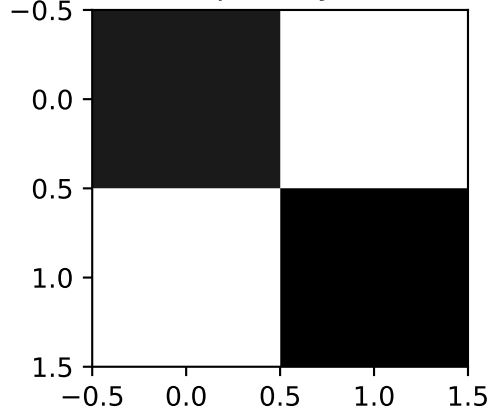
susceptibility (ULA)
