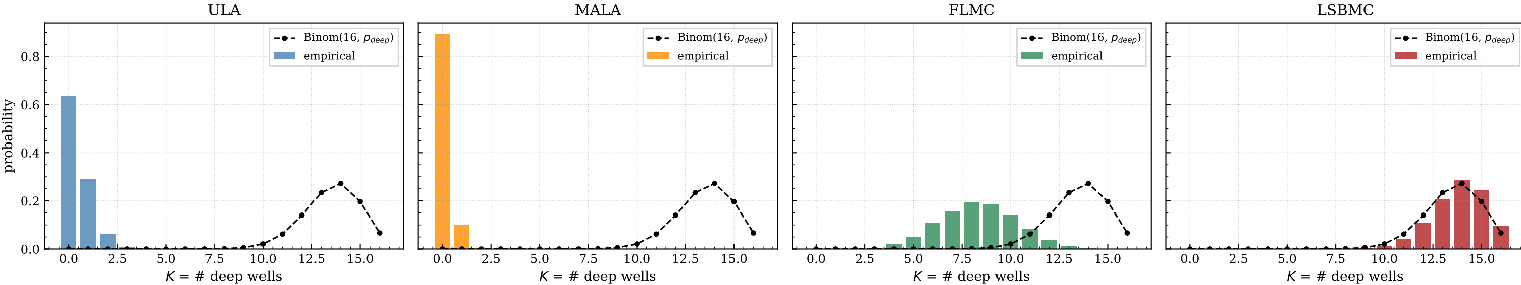
Final distribution of deep-well count K
