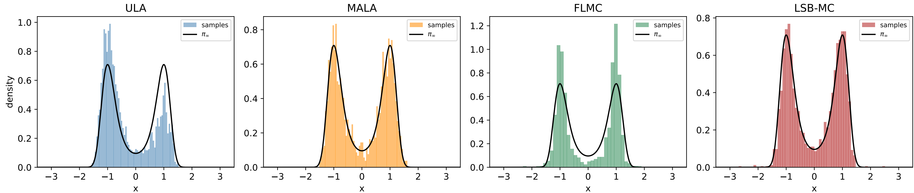
Final sample histograms vs \pi_\infty ( T = 20.0 )
