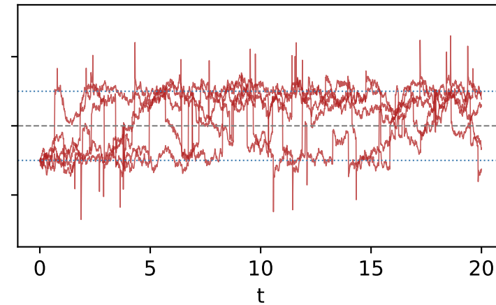
LSB-MC
