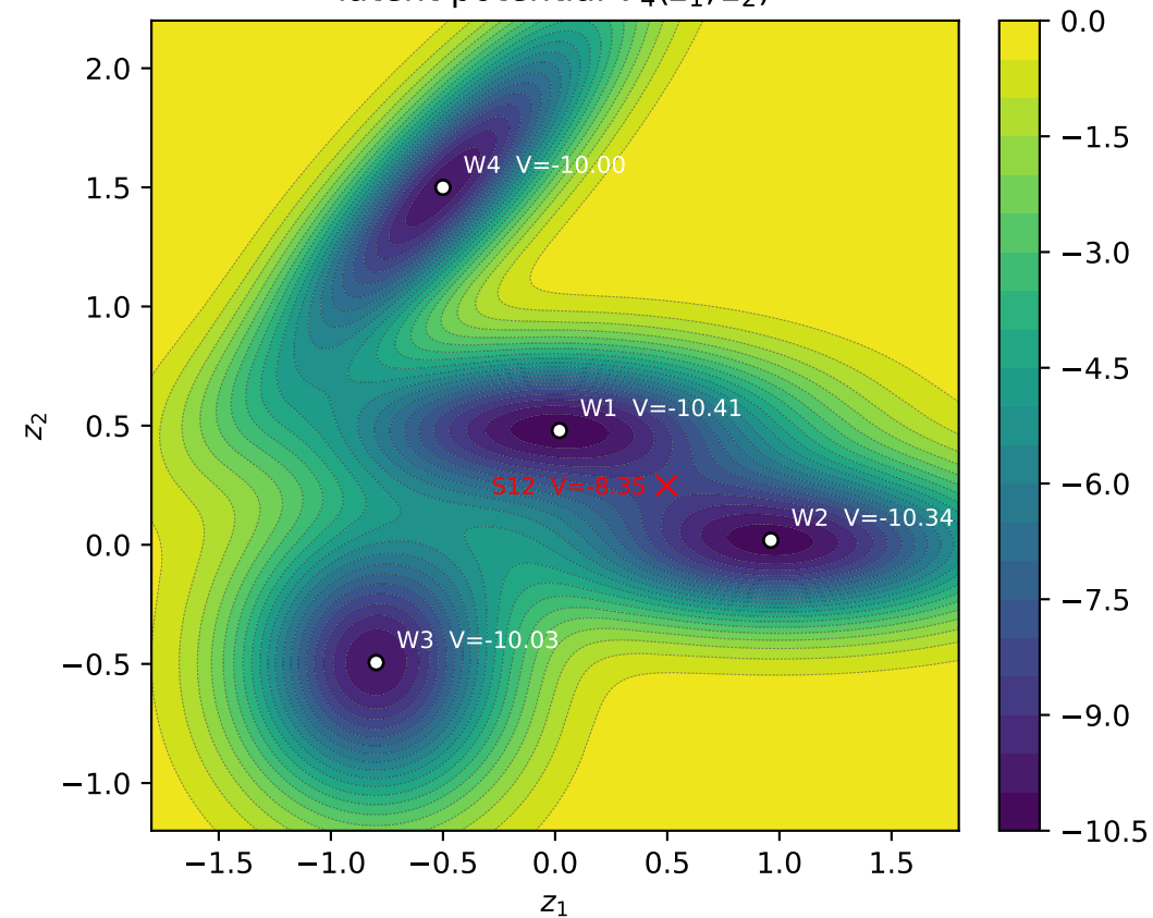
latent potential V_4(z_1, z_2)
