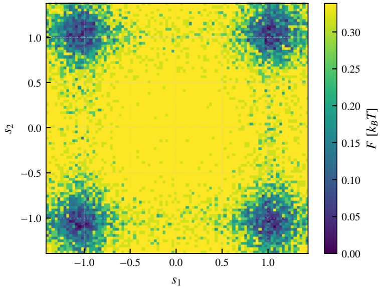
Raw-CP
