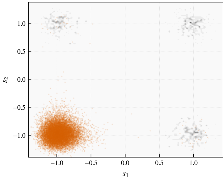
BAOAB vs reference (shaded)
