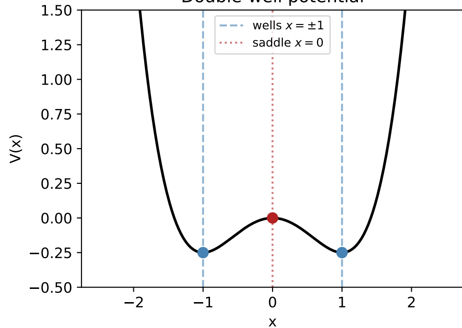
Double-well potential
