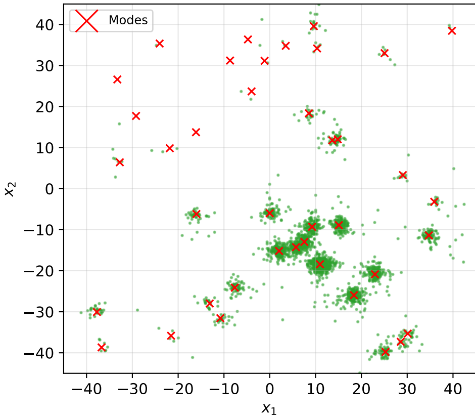
MoG40: FLMC (EMC=0.38, Cov=92%)
