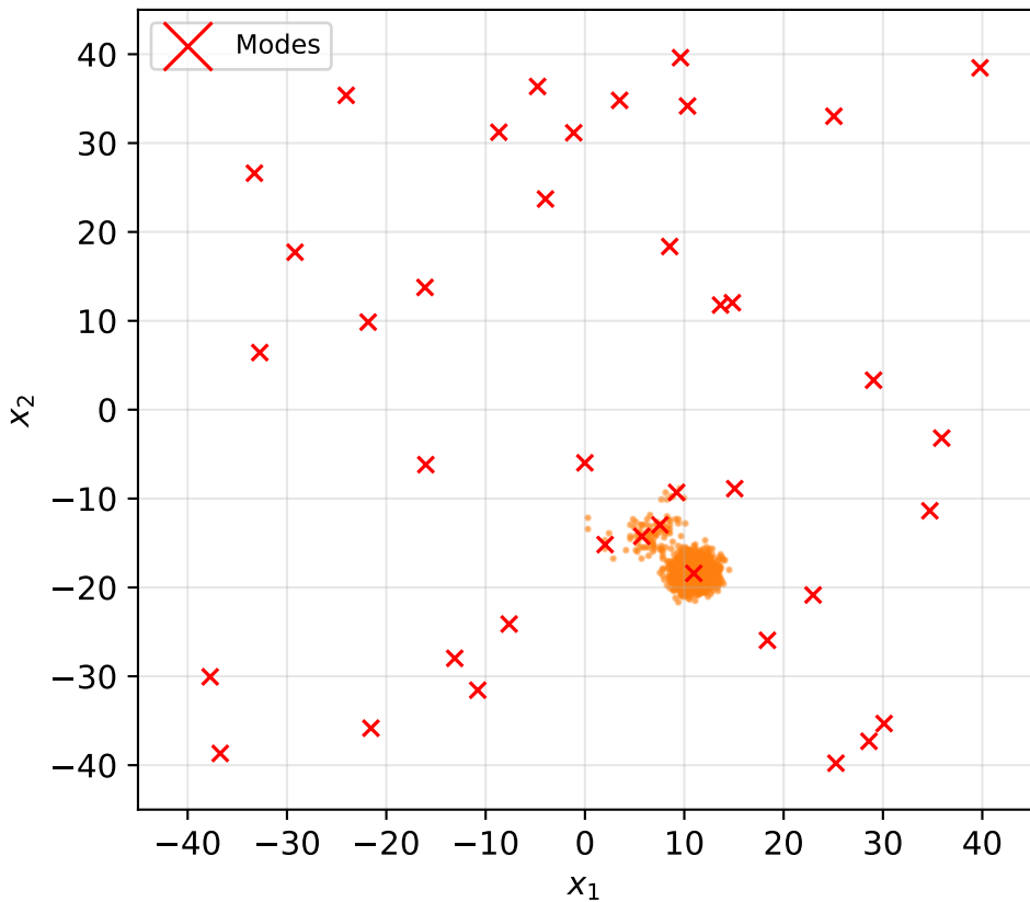
MoG40: MALA (EMC=0.03, Cov=12%)
