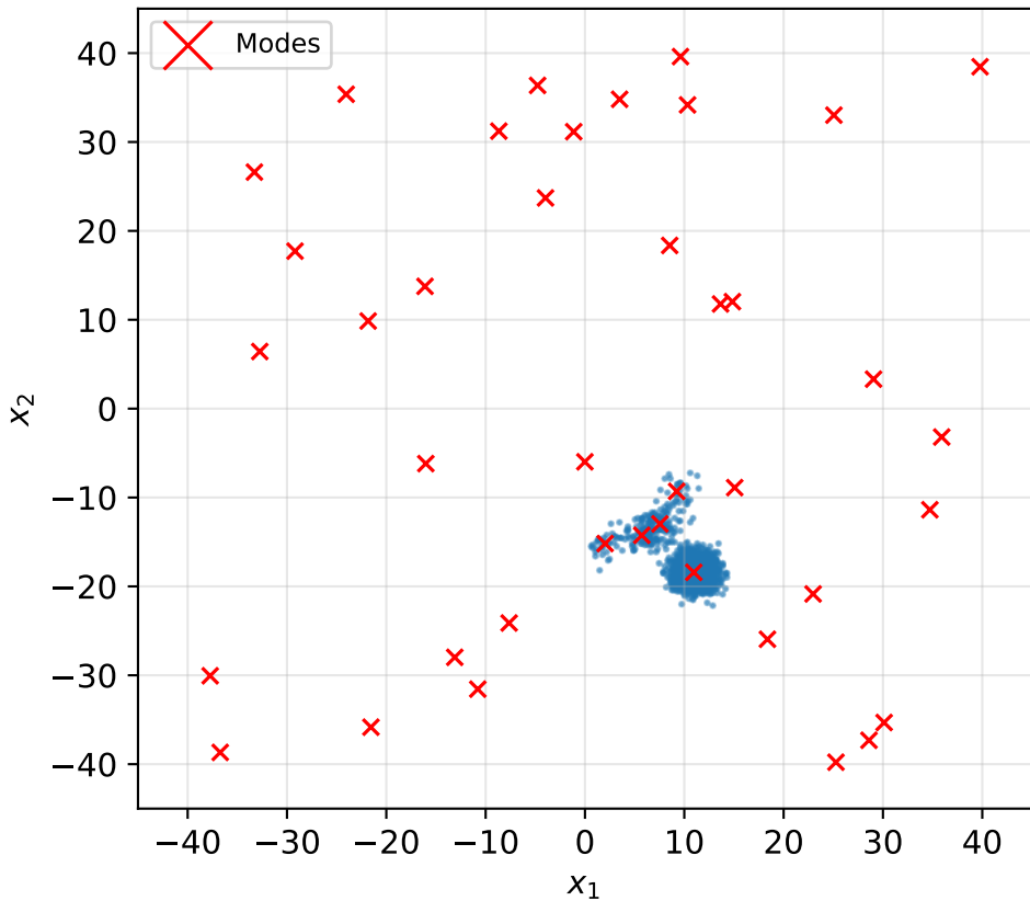
MoG40: ULA (EMC=0.04, Cov=12%)
