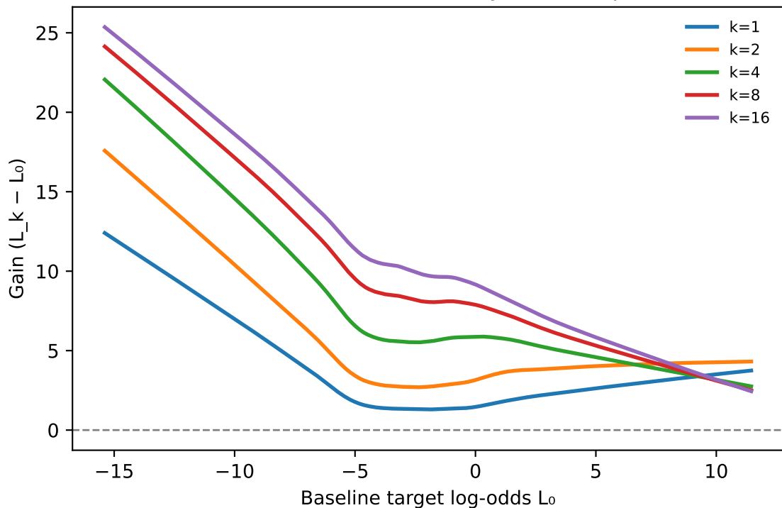
Gain vs baseline (LOWESS by relearn update)
