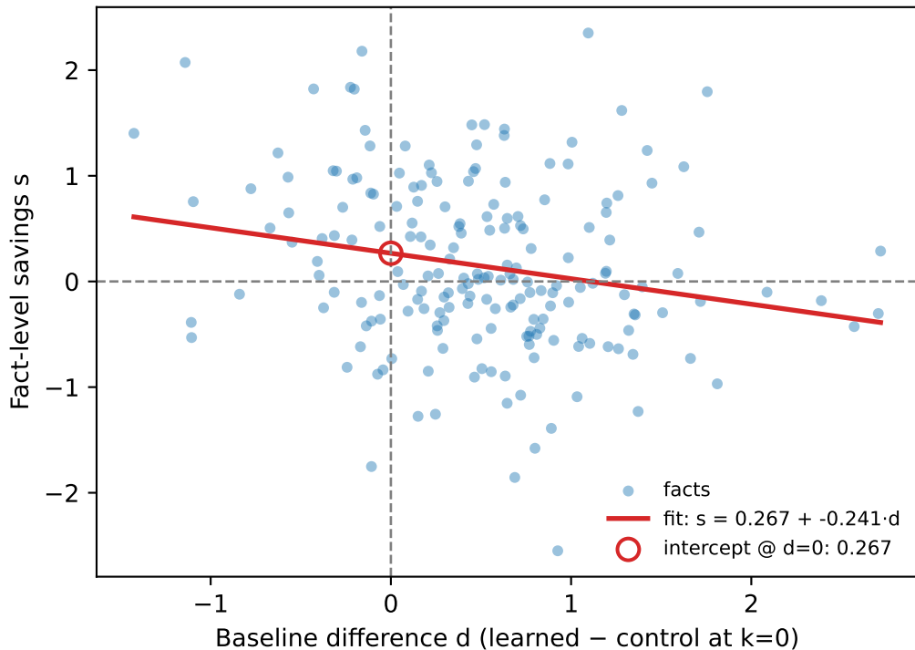
s vs d @ trough (learned_vs_control, seed 1)
