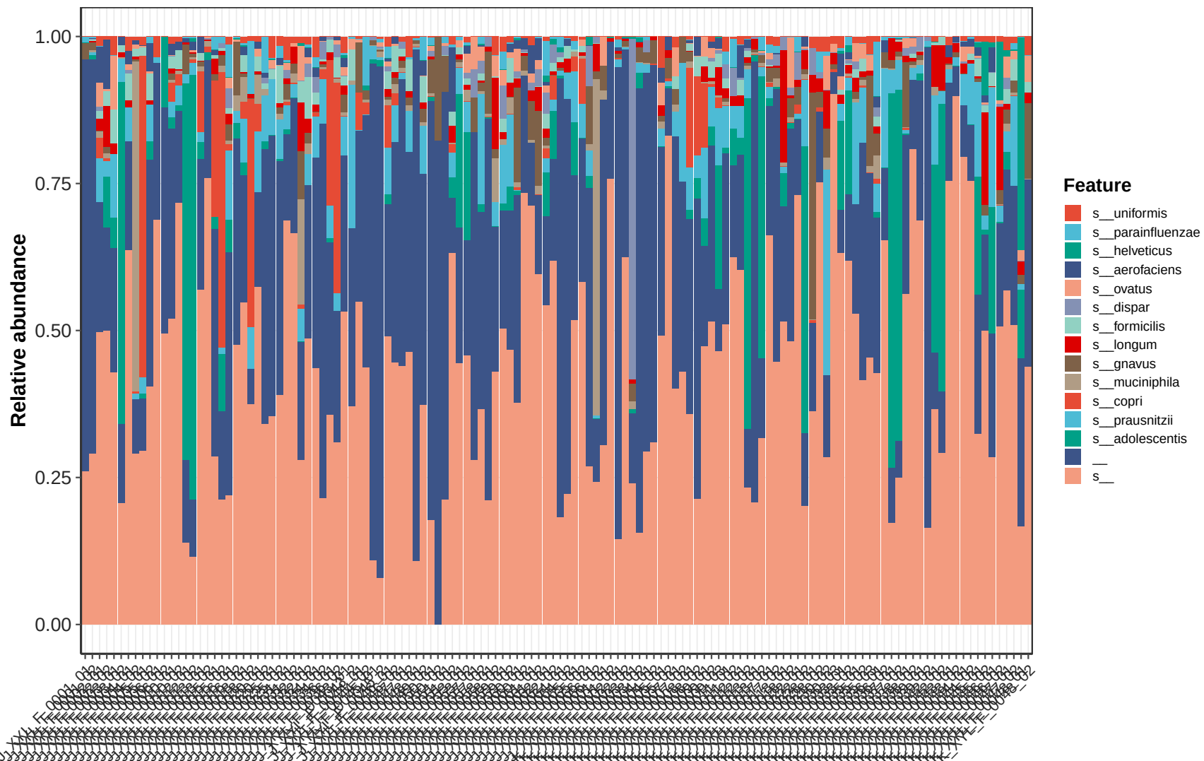
Top 15 features (relative abundance)
