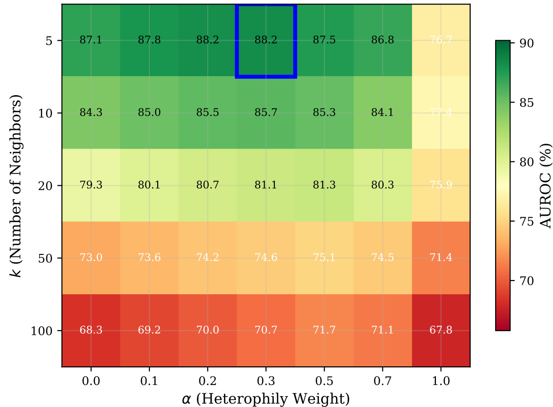
AUROC (%) Grid Search - Banking77
