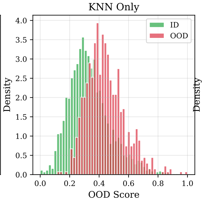
Score Distribution - Banking77
