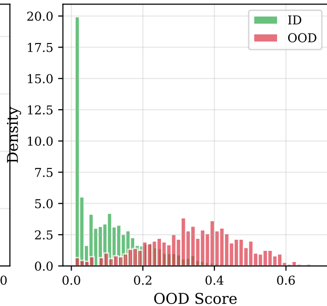
Heterophily Only
