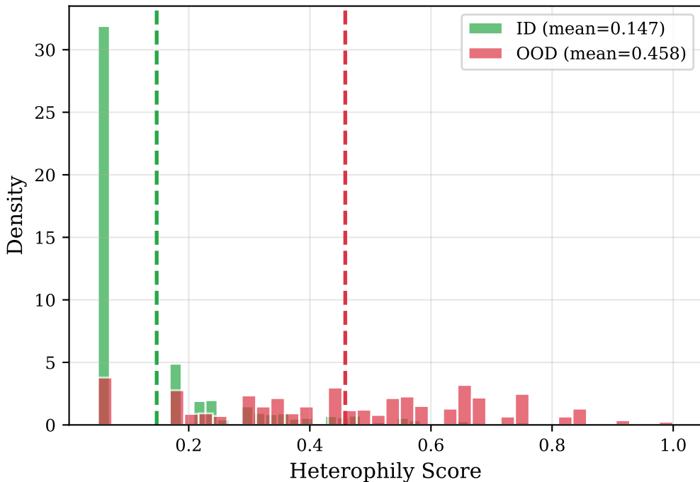
Heterophily Distribution - CLINC150
