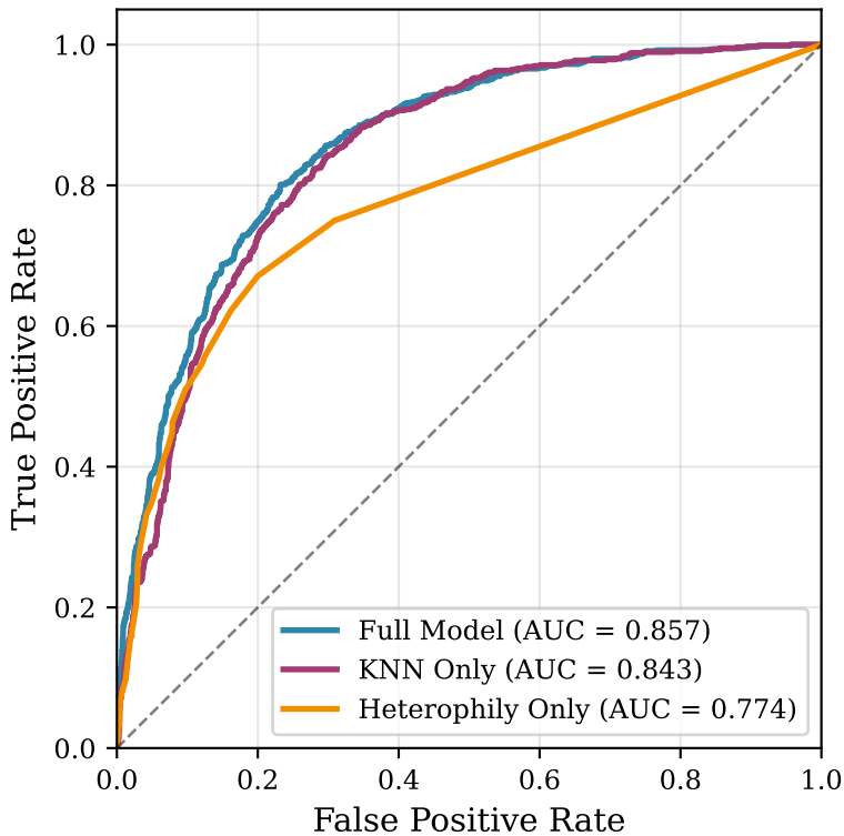
ROC Curves - Banking77
