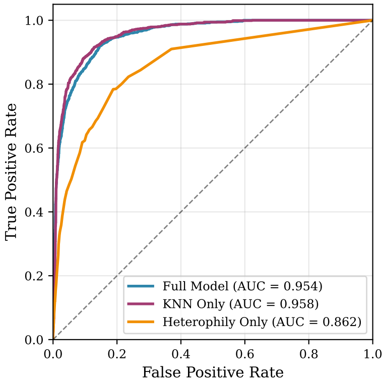
ROC Curves - CLINC150
