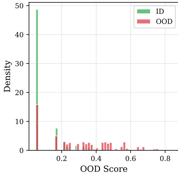
Heterophily Only
