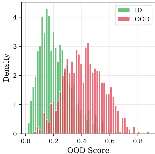
Full Model
