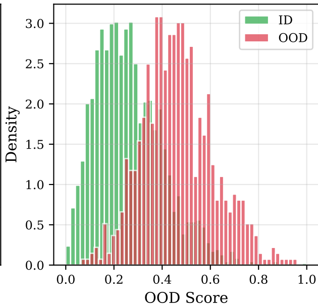
KNN Only
