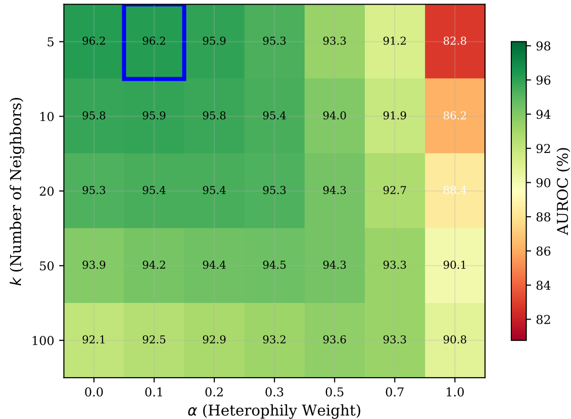
AUROC (%) Grid Search - CLINC150
