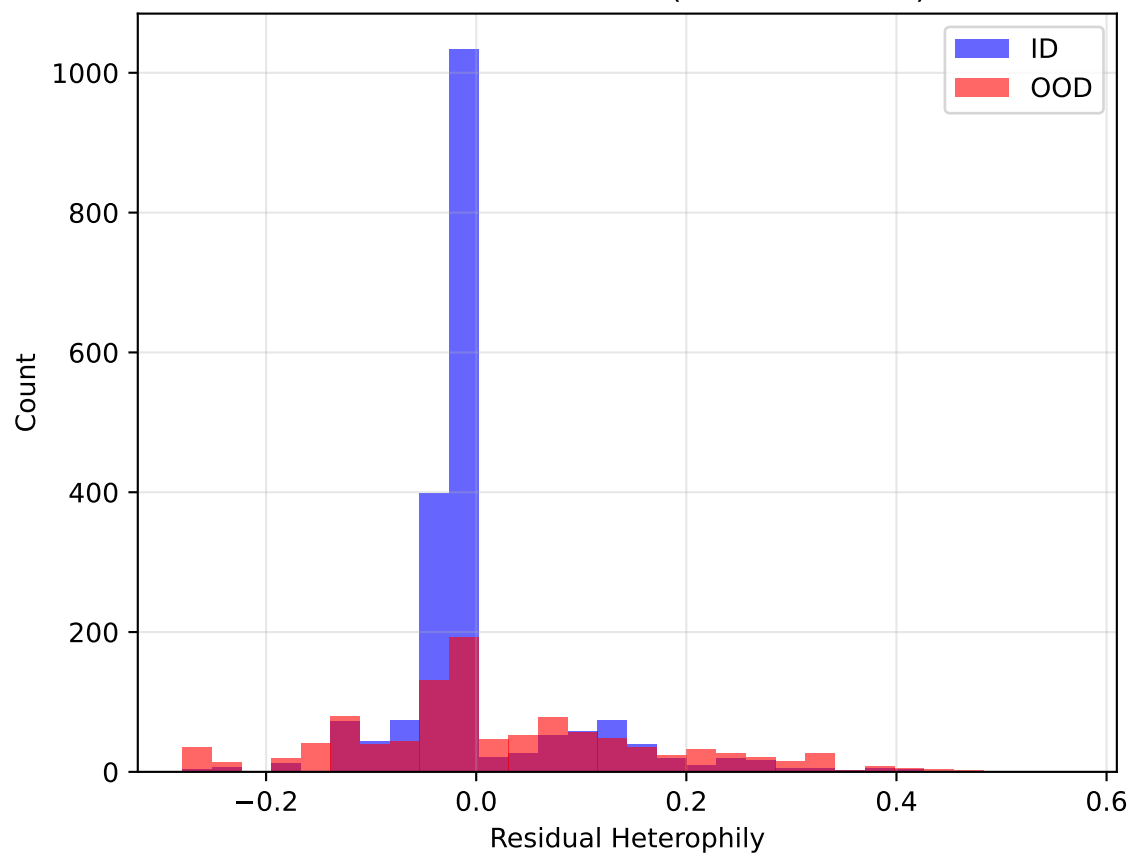
Residual Distribution (AUROC=0.544)
